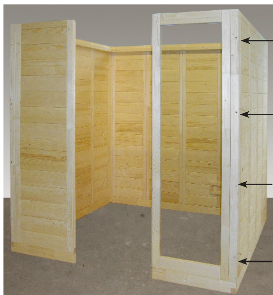
4 screws 6 x 100 mm
