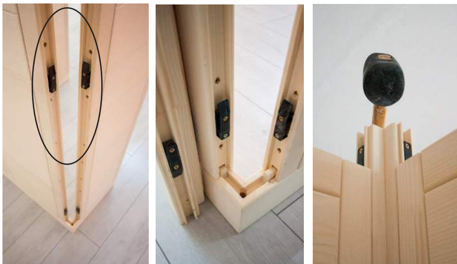
Fig. 4: Connecting wall elements with corner post
